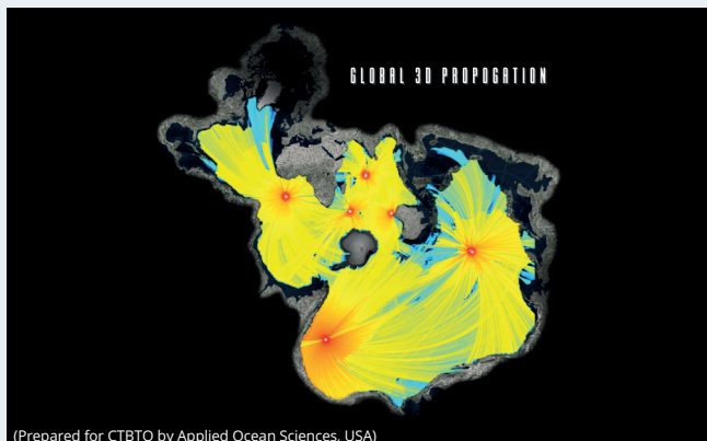
3-D underwater sound propagation simulation illustrating the acoustic coverage (red for high and blue for low detection capability) with IMS hydroacoustic hydrophone stations across the world's oceans, in Spilhaus Projection centered on Antarctica.
