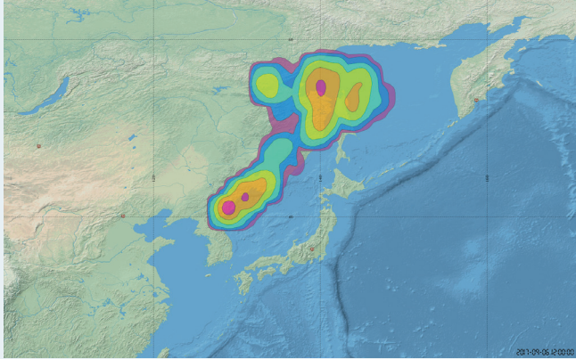
Snapshot illustrating the plume dispersion 3.5 days after the DPRK event on 3 September 2017. Simulation based on NCEP analysed data.
