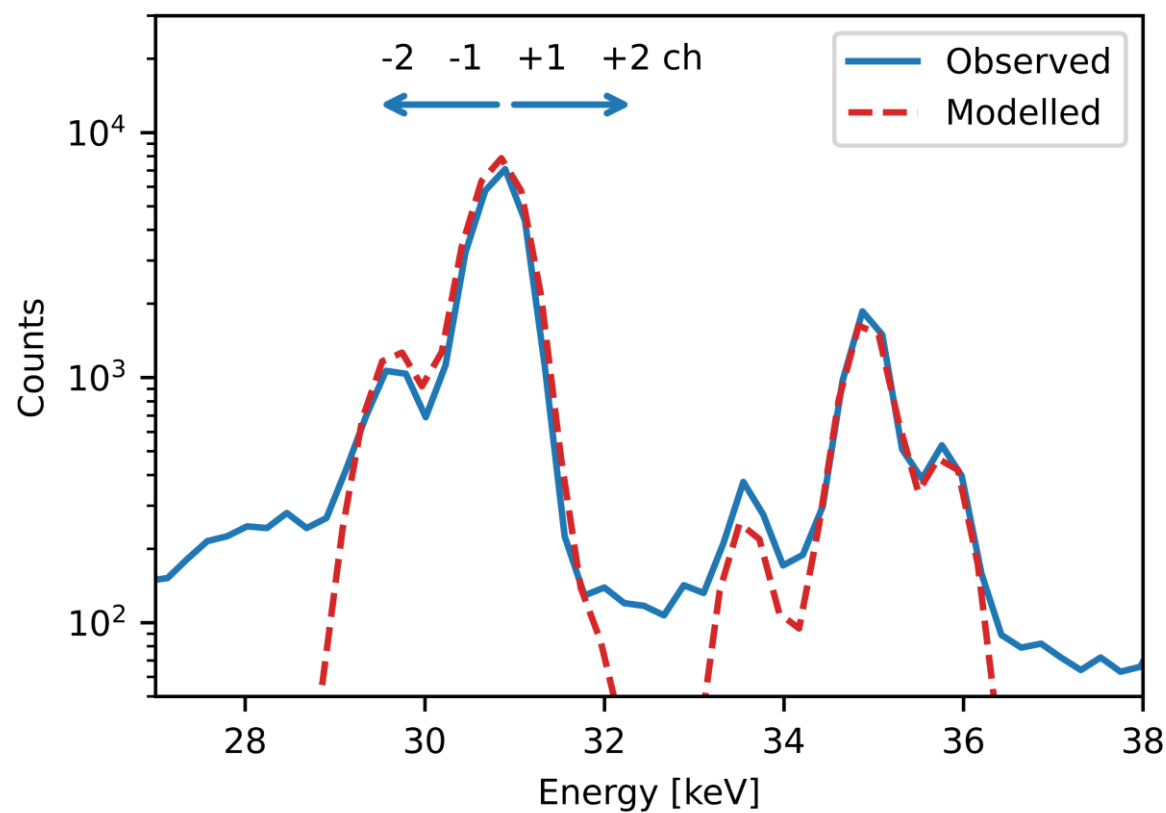
X-Ray Lorentzian Multiplets from Four Xenon Isotopes
