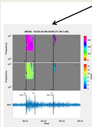
New event detected along Mohn ridge
