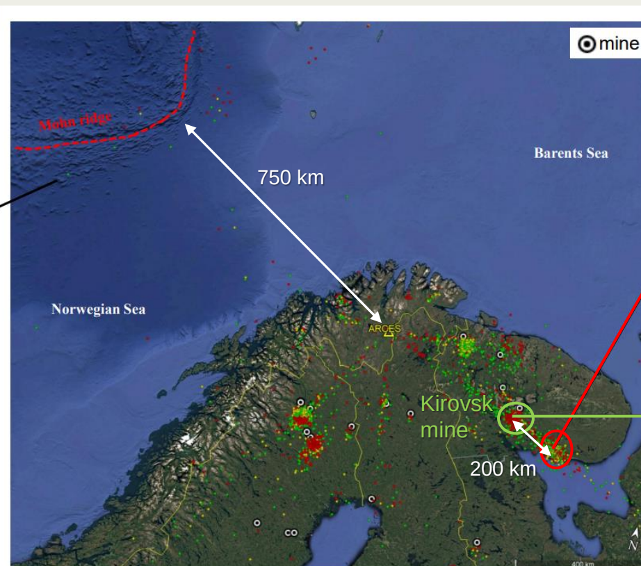
Map of detected events (dots) over one month of data, red corresponds to elos3c, yellow to elos1C and green to elos1C with denoising process.
