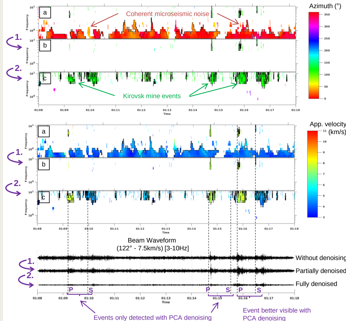
Figure: PCA denoising example using ARCES array. PMCC results obtained on raw data (a), partially denoised data (b), and fully denoised data (c). The top part presents the azimuth of coherent detections, the middle the apparent velocity, and the bottom the array beam waveform.
