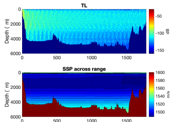
Figure: TL and SSPs for a 8 m source depth at (5.92^\circ, 81.131^\circ) off the southern coast of Sri Lanka.
