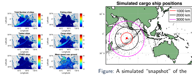
Figure: Total number of ships in December 2014 at a resolution of 0.25^\circ \times 0.25^\circ ( exactEarth Ltd.).
