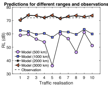
Figure: Predictions and Observations
