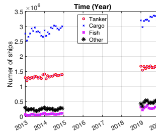
Figure: Total number of ships in 2000 km radius around Diego Garcia (S).
