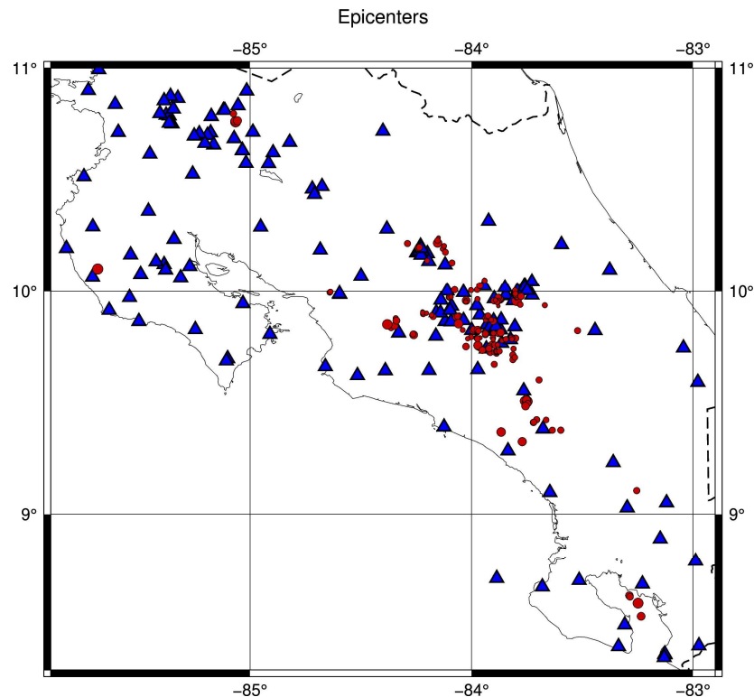
Fig. 1. The figure shows GT5 candidates represented by red circles and seismic stations that recorded them represented by blue triangles, a total 178 events were identified.
